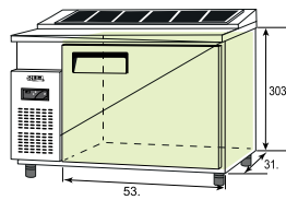
Interior dimensions
